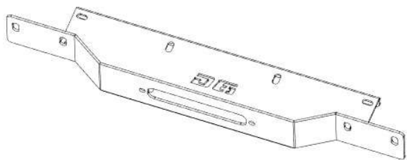
Winch plate
