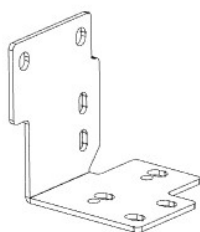
Side bracket
